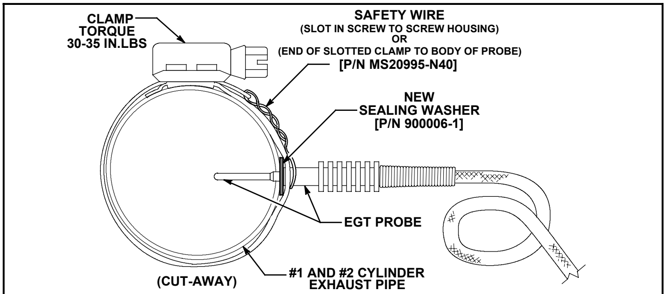
Figure SB M20-311-2 - EXHAUST GAS TEMPERATURE PROBE AND COMPONENTS
