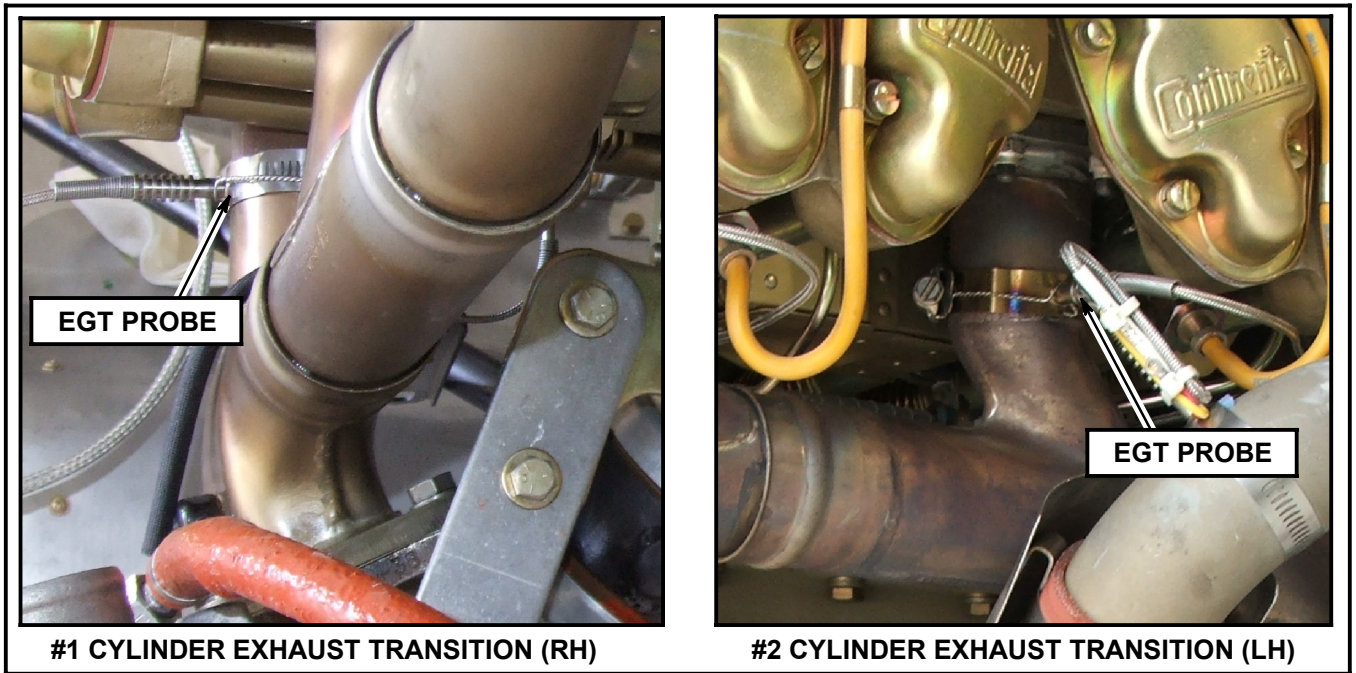
Figure SB M20-311-1 - EXHAUST GAS TEMPERATURE PROBE LOCATION
