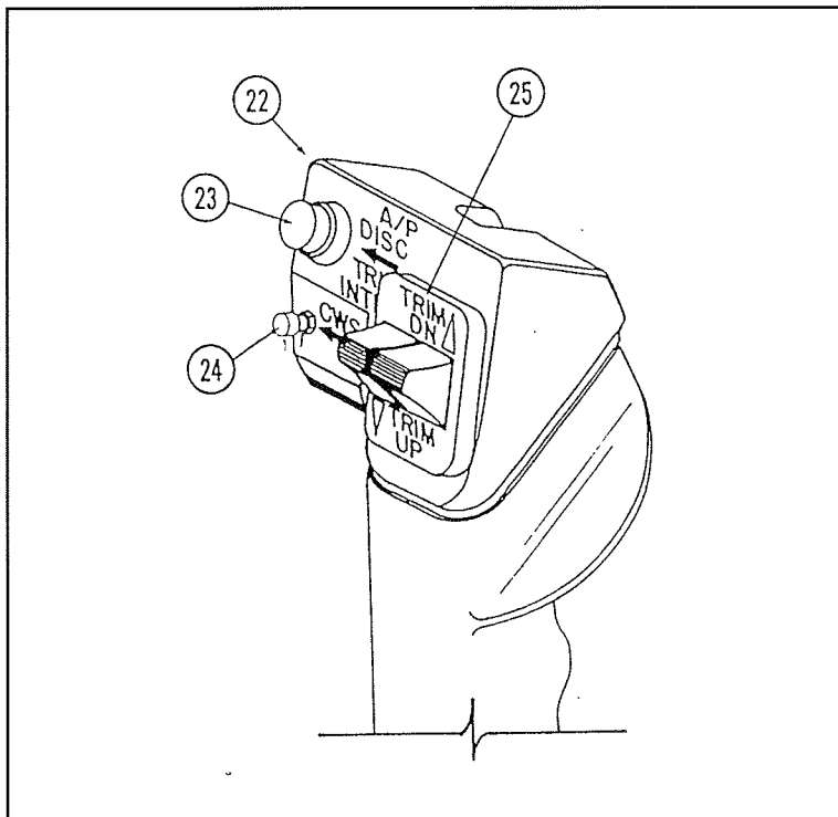
FIGURE 3 - A/P CONTROL WHEEL SWITCH CAP
