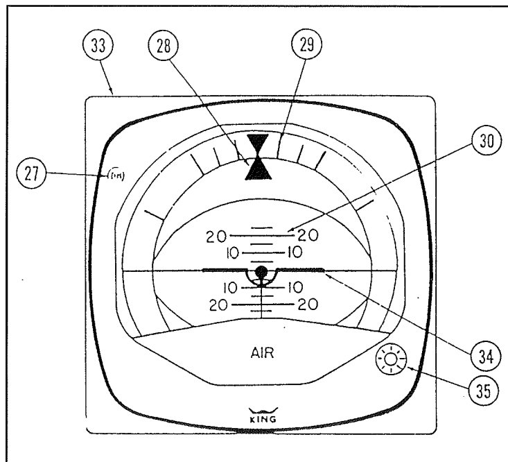
FIGURE 5 - KG 258 VERTICAL GYRO
