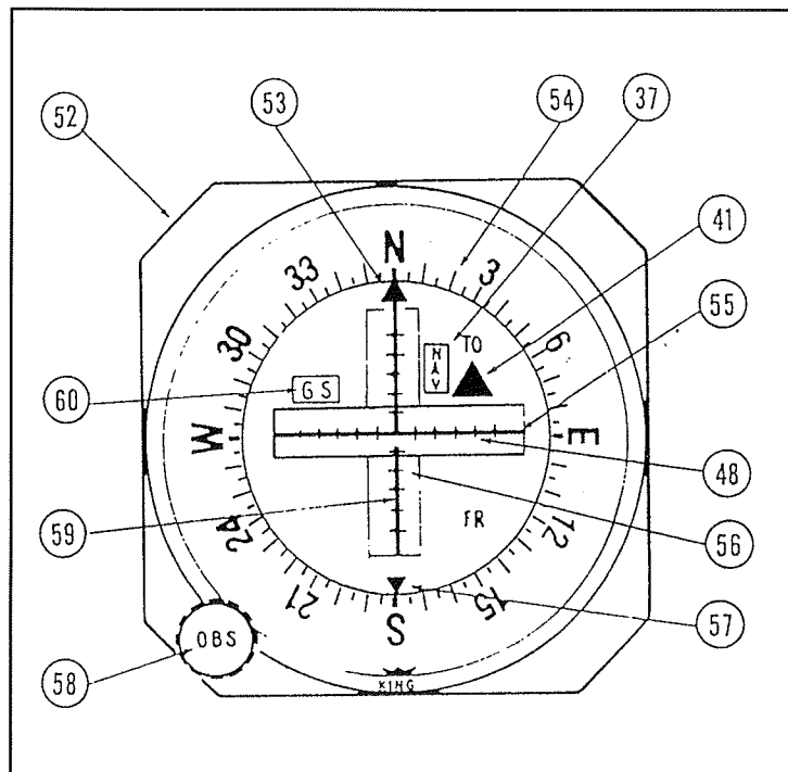
FIGURE 8 - KI 204/206 VOR/LOC/GS INDICATOR
