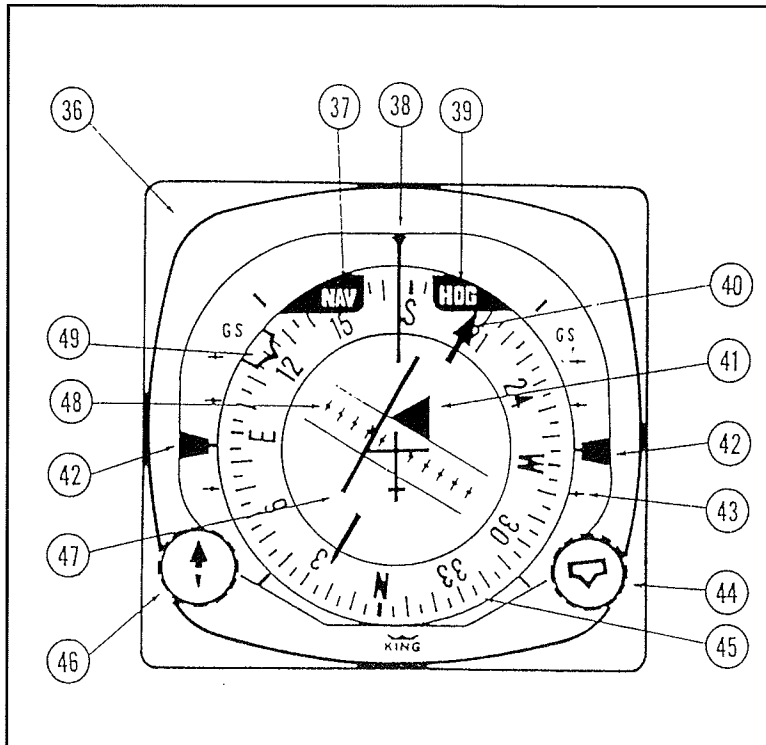
FIGURE 6 - KI 525A HSI
