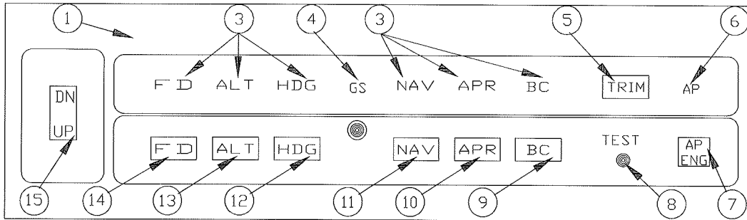
FIGURE 1 - KC 192 AUTOPILOT & FLIGHT DIRECTOR COMPUTER
