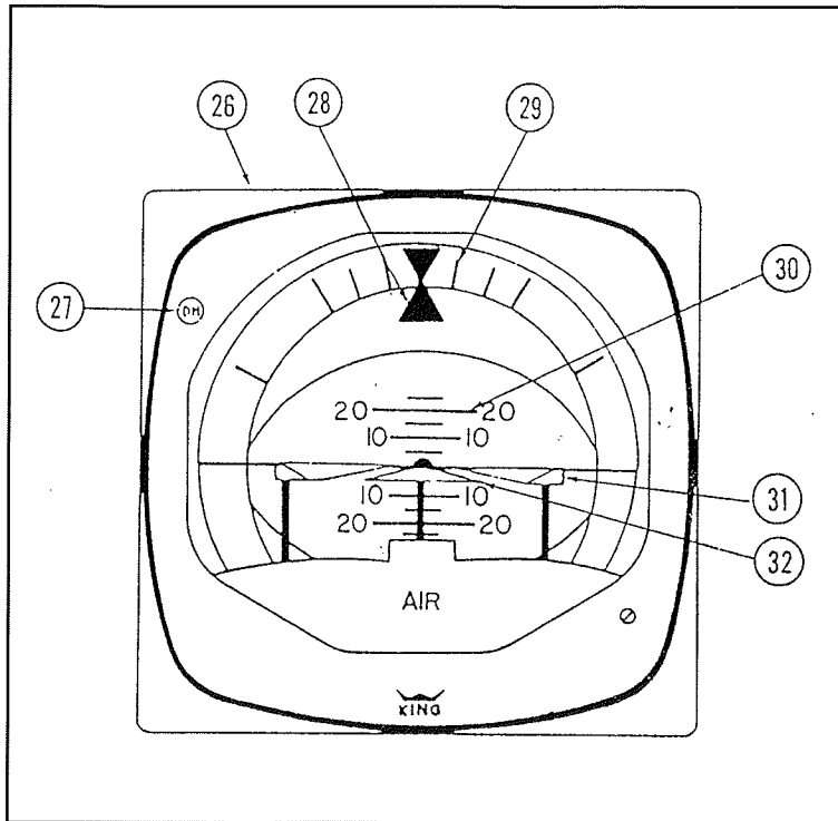
FIGURE 4 - KI 256 FLIGHT COMMAND INDICATOR
