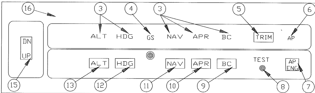
FIGURE 2 - KC 191 AUTOPILOT COMPUTER
